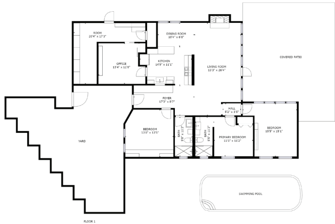
GROSS INTERNAL AREA FLOOR 1: 1729 sq. ft. TOTAL: 1729 sq. ft. DIMENSIONS AND DEPENDENCIES ARE APPROXIMATE, ACTUAL MAY VARY.
